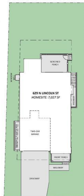
629 N LINCOLN ST | SCHEMATIC SITE PLAN
