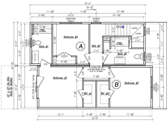
Second Floor Plan SCALE: 3/16" = 1'-0"
