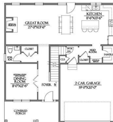
FIRST FLOOR PLAN: AREA = 1,130 S.F.
